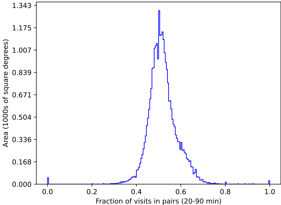
ddf_loaded_fl4_v3.4_10yrs gri All sky: Fraction of visits in pairs (20-90 min)
