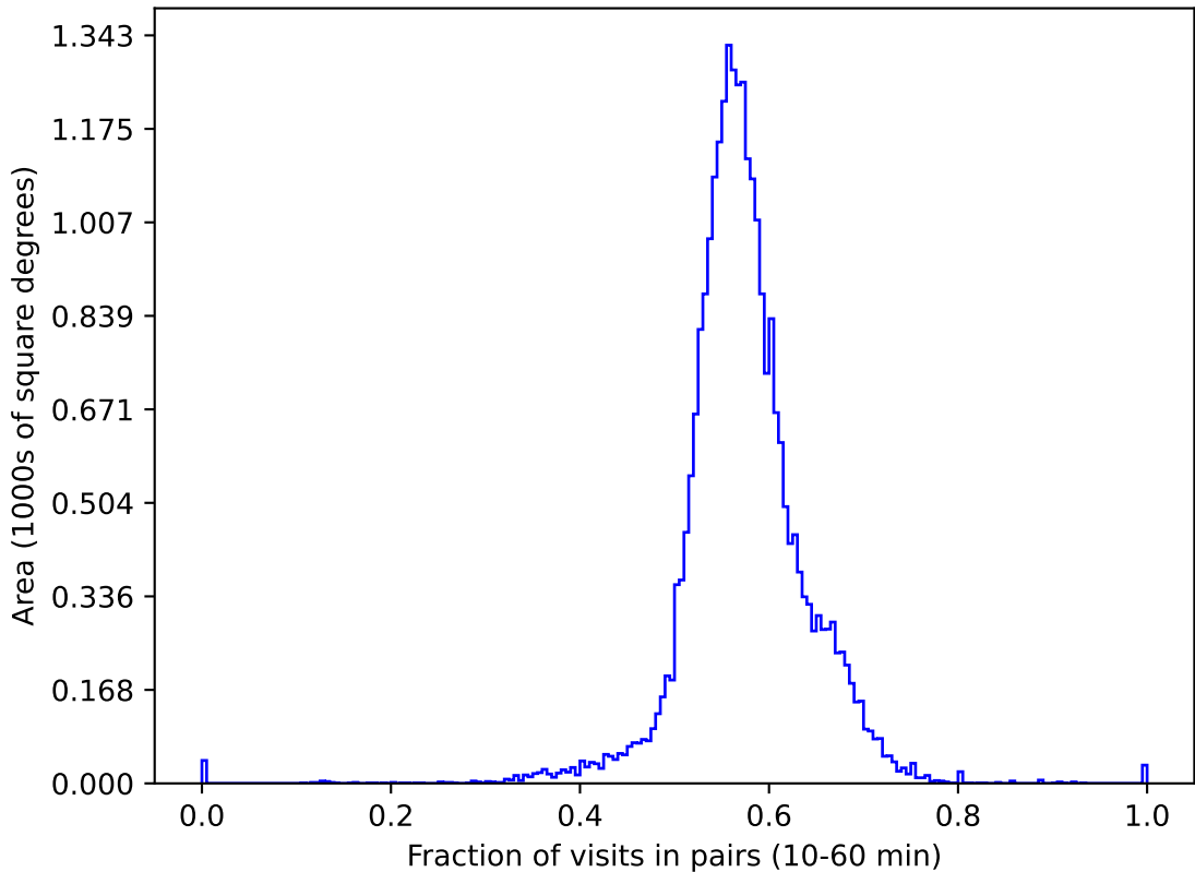
ddf_loaded_fl4_v3.4_10yrs gri All sky: Fraction of visits in pairs (10-60 min)
