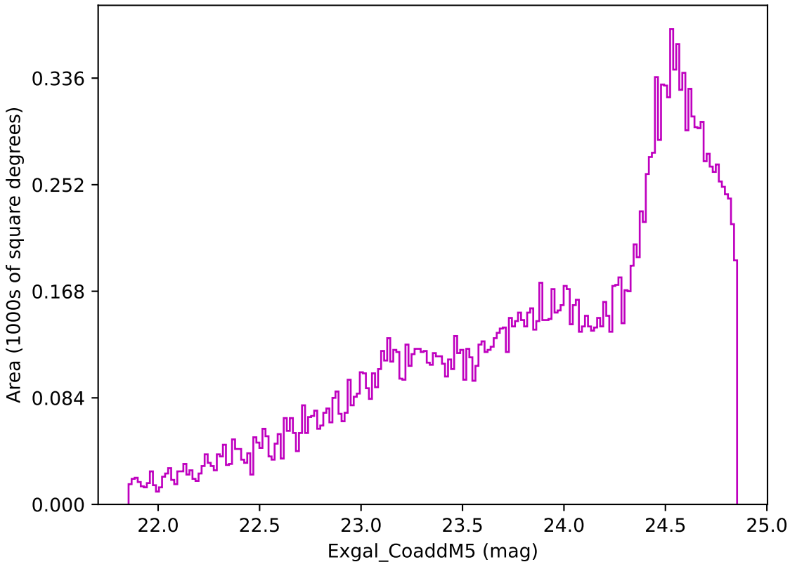
ddf_loaded_fl4_v3.4_10yrs Yr 3-4 z band: Exgal_CoaddM5
