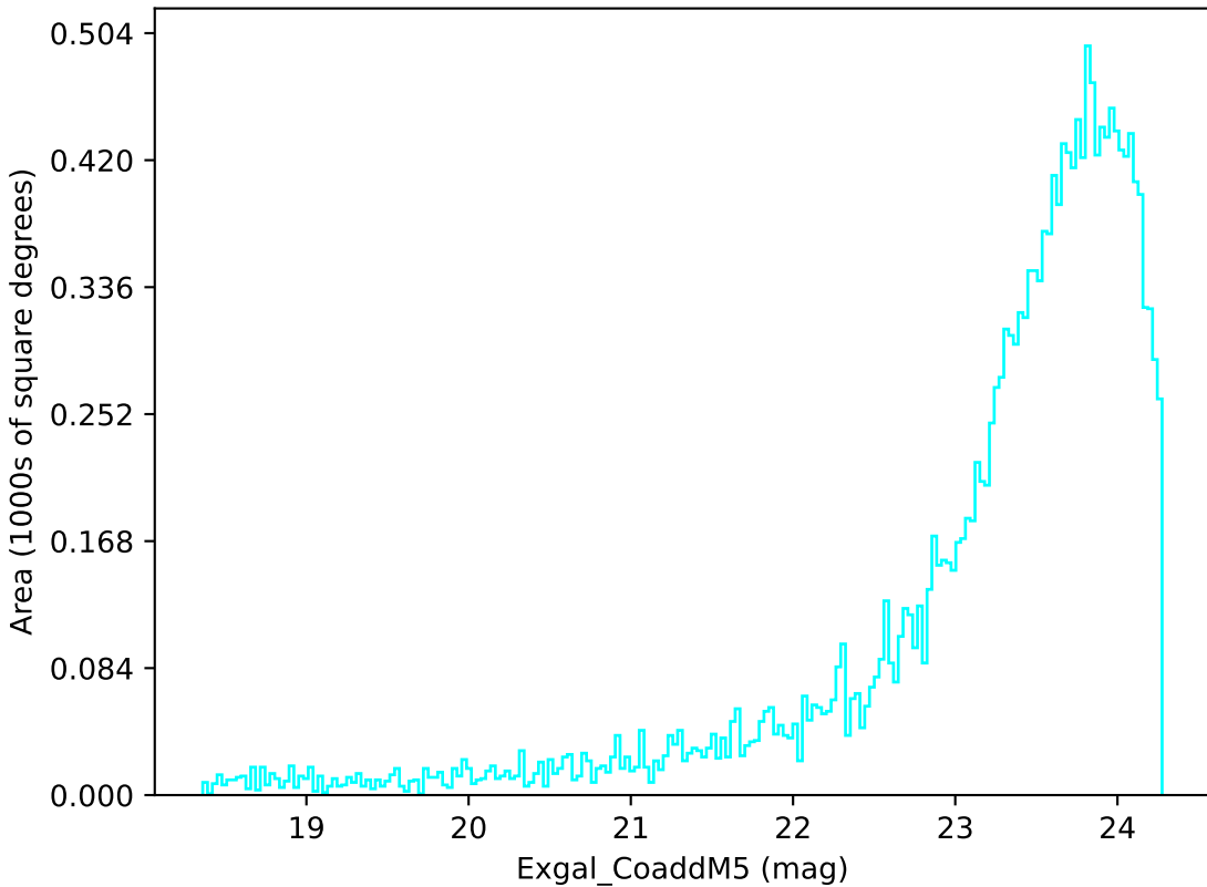
ddf_loaded_fl4_v3.4_10yrs Yr 3-4 u band: Exgal_CoaddM5
