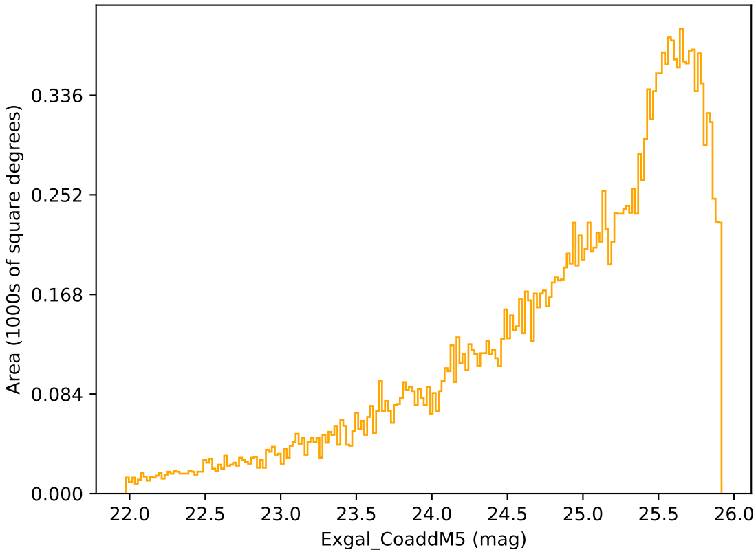
ddf_loaded_fl4_v3.4_10yrs Yr 3-4 r band: Exgal_CoaddM5
