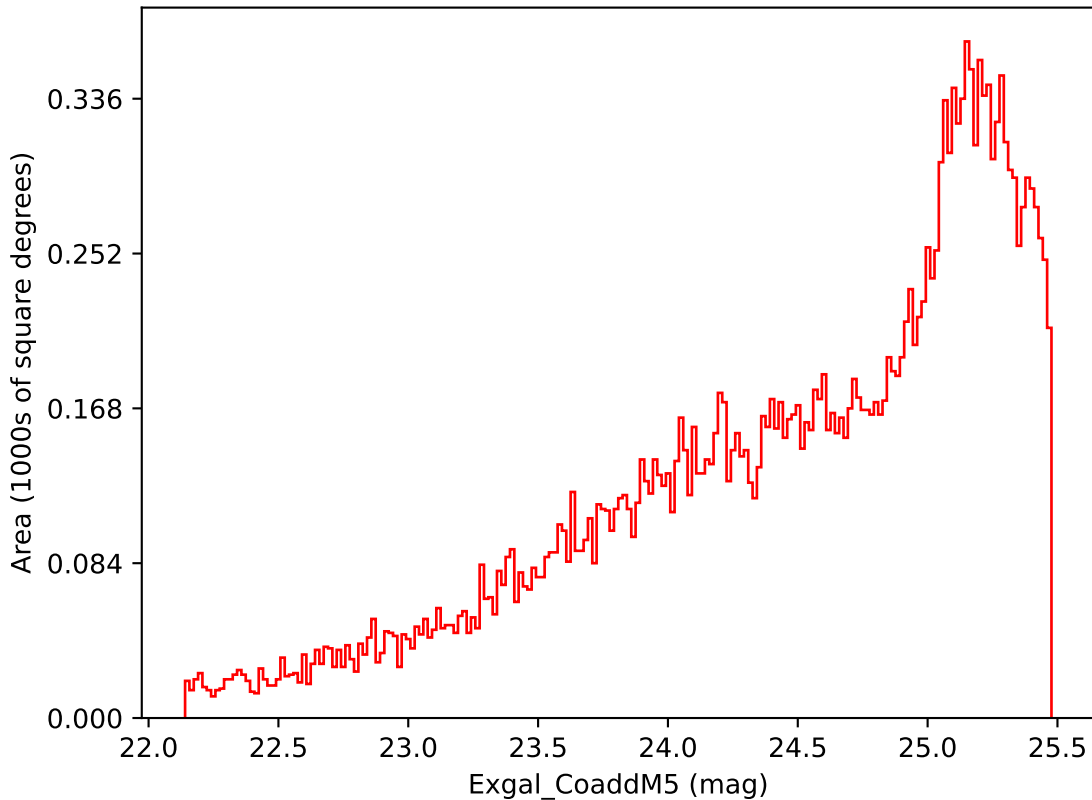
ddf_loaded_fl4_v3.4_10yrs Yr 3-4 i band: Exgal_CoaddM5
