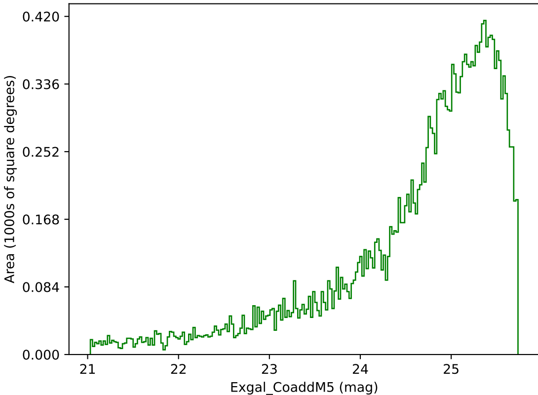
ddf_loaded_fl4_v3.4_10yrs Yr 3-4 g band: Exgal_CoaddM5
