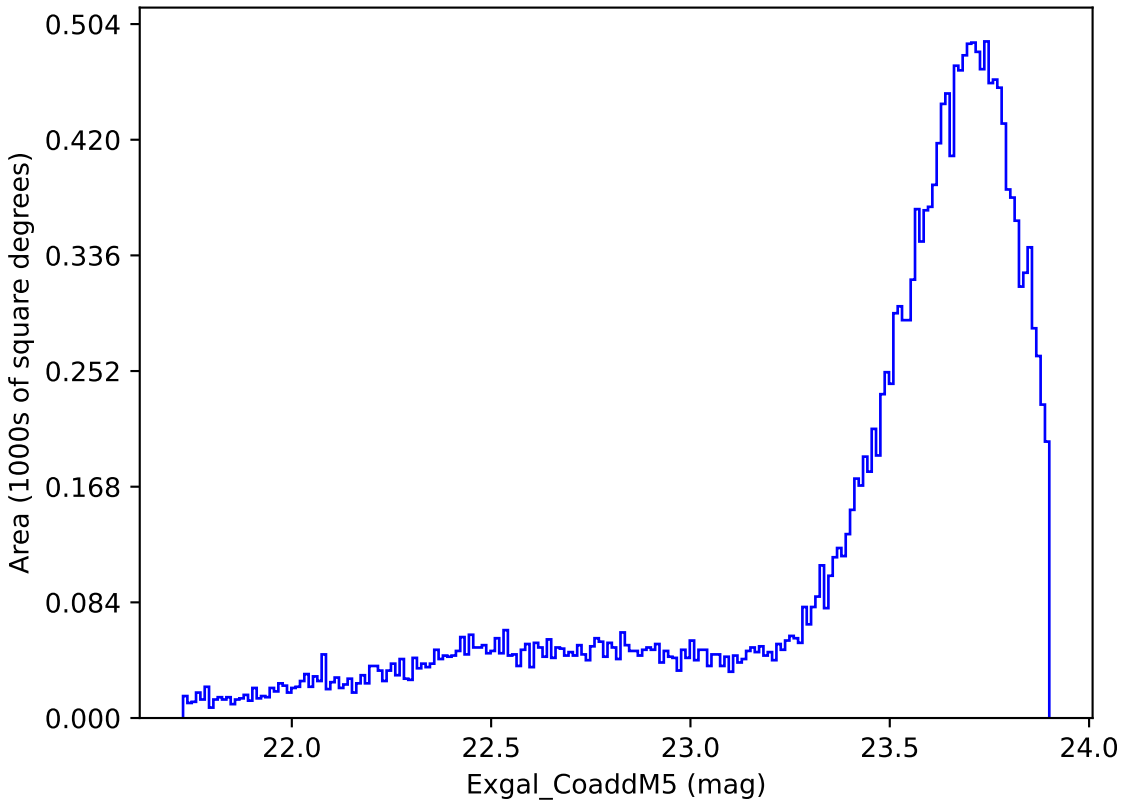
ddf_loaded_fl4_v3.4_10yrs Yr 1 y band: Exgal_CoaddM5
