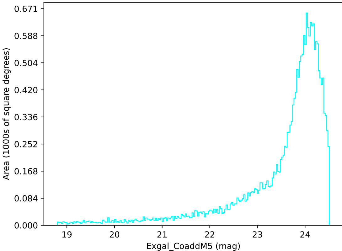
ddf_loaded_fl4_v3.4_10yrs Yr 1 u band: Exgal_CoaddM5
