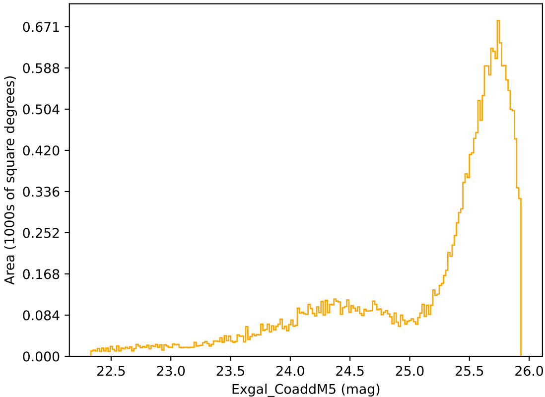
ddf_loaded_fl4_v3.4_10yrs Yr 1 r band: Exgal_CoaddM5
