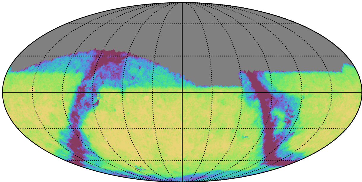
ddf_loaded_fl4_v3.4_10yrs Yr 1 i band: Exgal_CoaddM5
