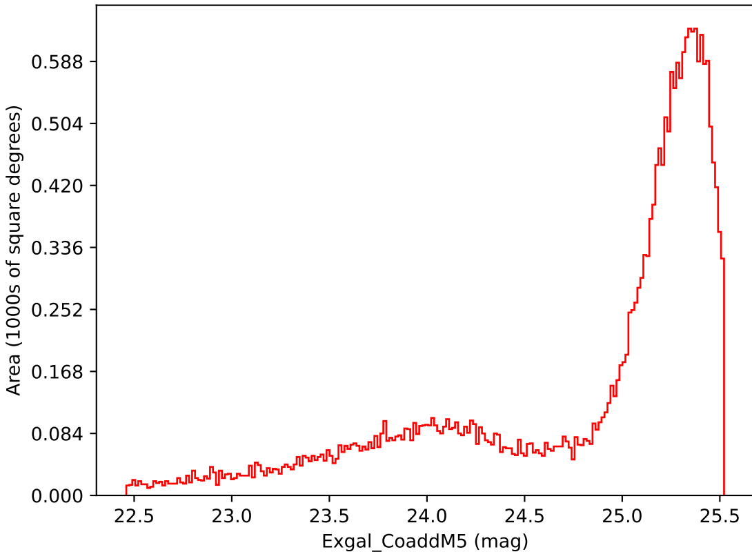
ddf_loaded_fl4_v3.4_10yrs Yr 1 i band: Exgal_CoaddM5
