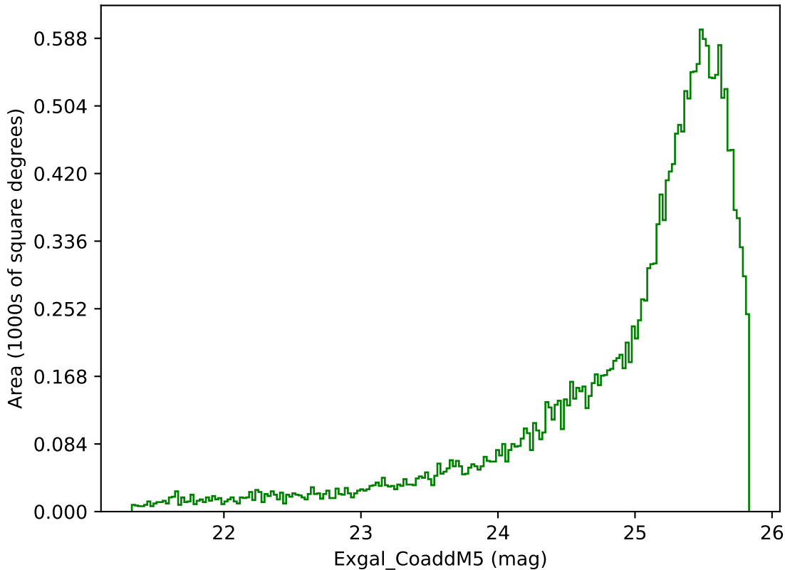
ddf_loaded_fl4_v3.4_10yrs Yr 1 g band: Exgal_CoaddM5
