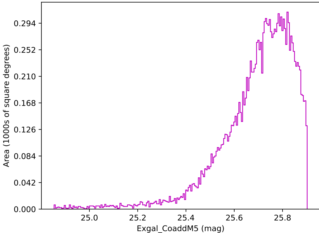
ddf_loaded_fl4_v3.4_10yrs WFD z band: Exgal_CoaddM5
