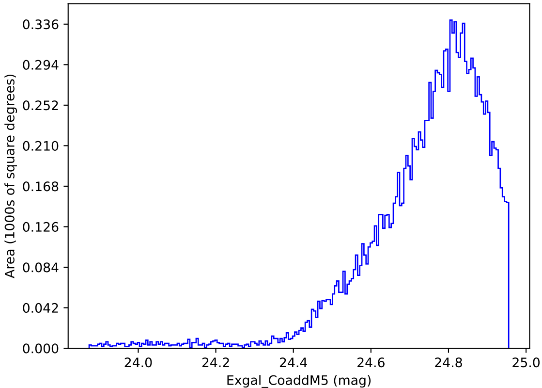
ddf_loaded_fl4_v3.4_10yrs WFD y band: Exgal_CoaddM5
