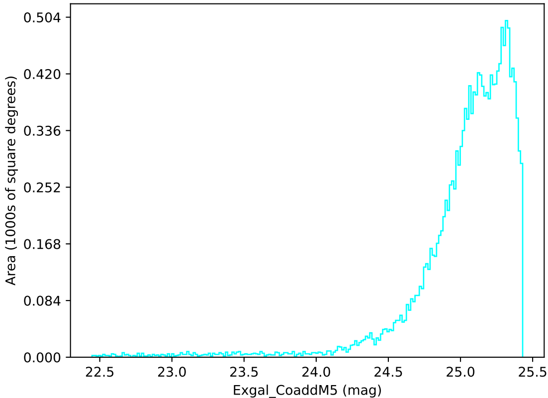
ddf_loaded_fl4_v3.4_10yrs WFD u band: Exgal_CoaddM5
