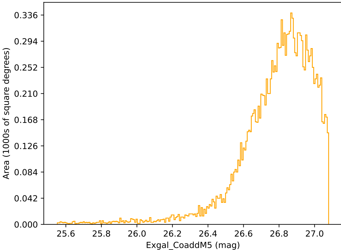
ddf_loaded_fl4_v3.4_10yrs WFD r band: Exgal_CoaddM5
