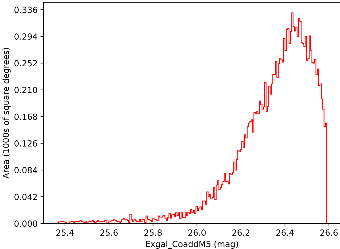
ddf_loaded_fl4_v3.4_10yrs WFD i band: Exgal_CoaddM5
