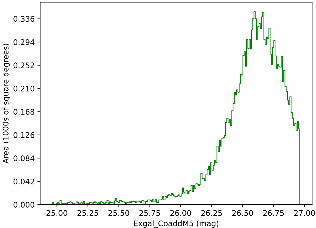
ddf_loaded_fl4_v3.4_10yrs WFD g band: Exgal_CoaddM5
