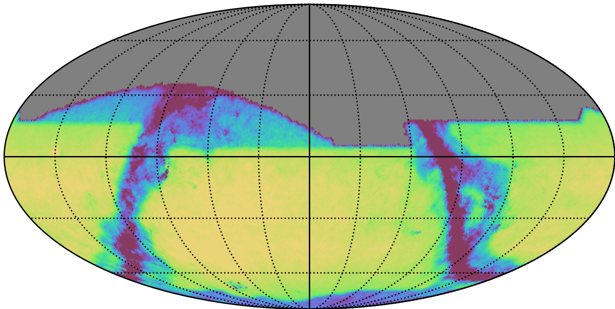
ddf_loaded_fl4_v3.4_10yrs All sky z band: Exgal_CoaddM5
