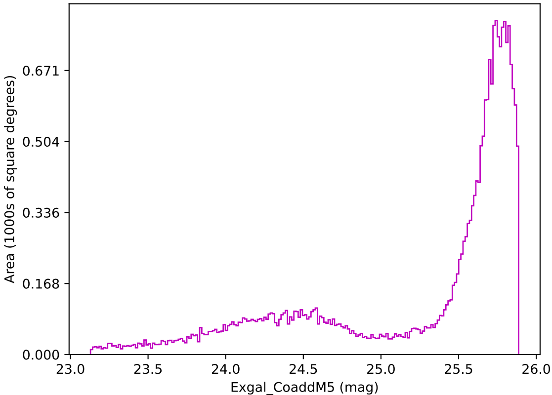
ddf_loaded_fl4_v3.4_10yrs All sky z band: Exgal_CoaddM5
