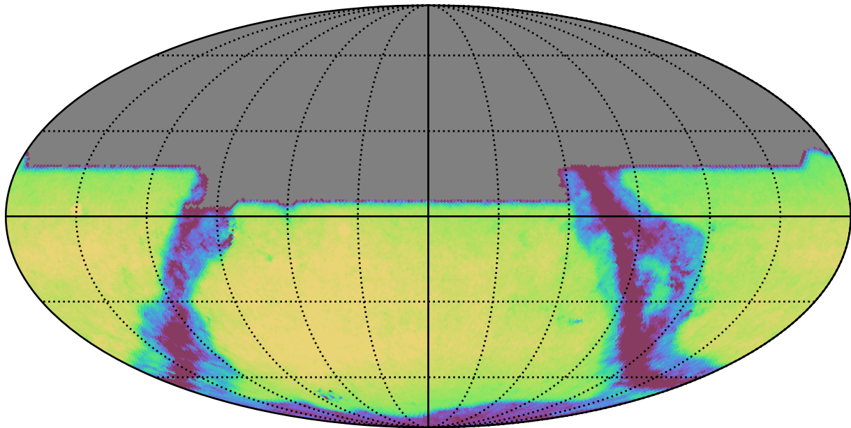
ddf_loaded_fl4_v3.4_10yrs All sky y band: Exgal_CoaddM5
