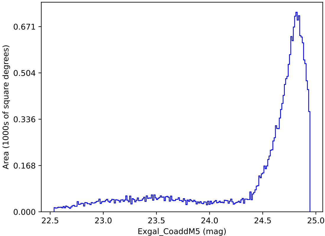
ddf_loaded_fl4_v3.4_10yrs All sky y band: Exgal_CoaddM5
