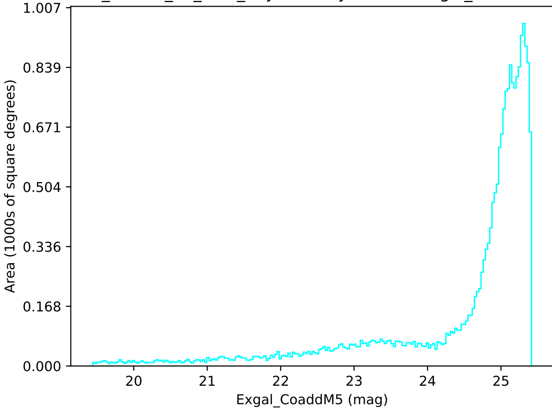
ddf_loaded_fl4_v3.4_10yrs All sky u band: Exgal_CoaddM5
