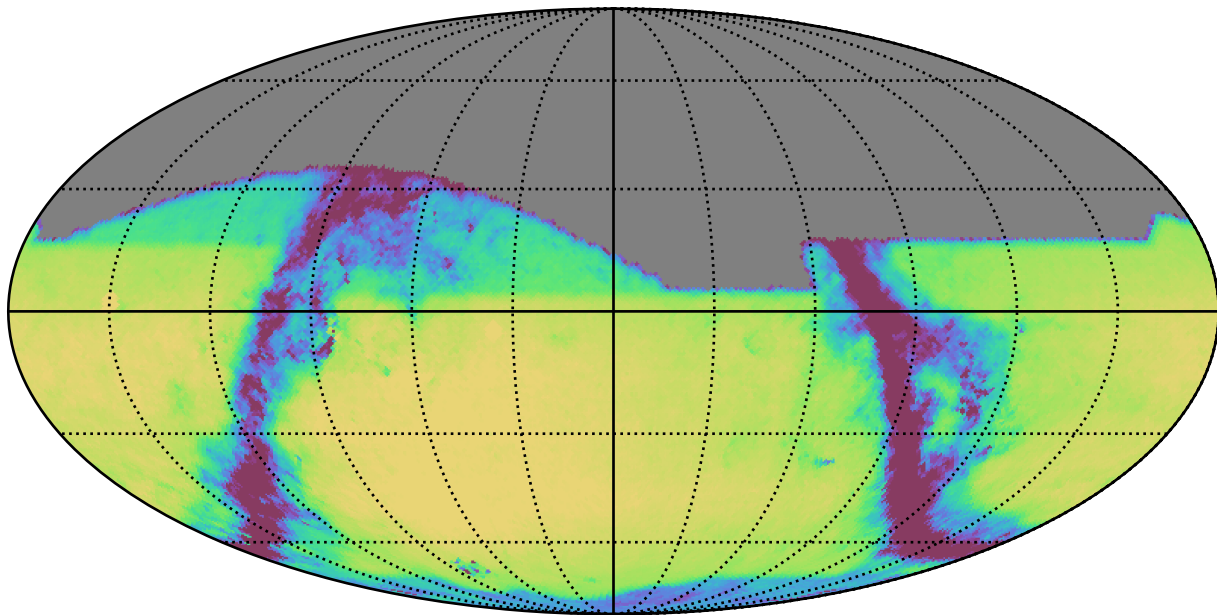
ddf_loaded_fl4_v3.4_10yrs All sky r band: Exgal_CoaddM5
