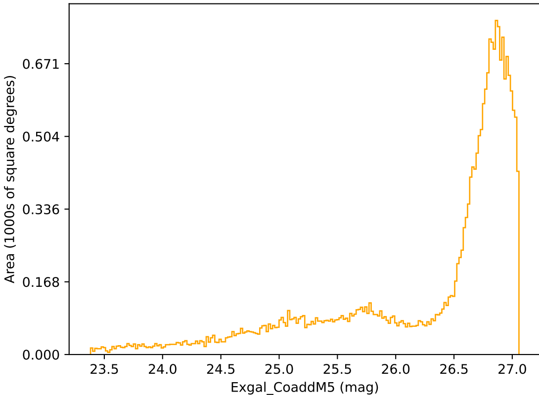
ddf_loaded_fl4_v3.4_10yrs All sky r band: Exgal_CoaddM5
