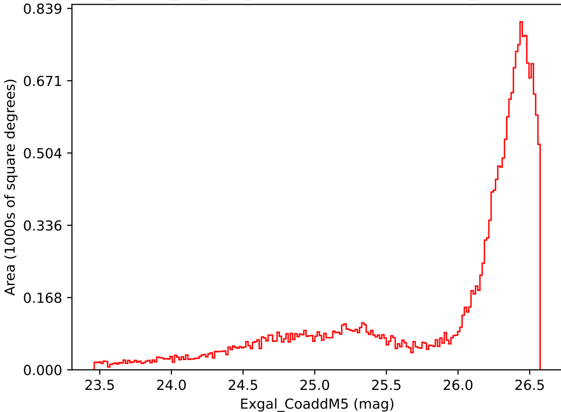
ddf_loaded_fl4_v3.4_10yrs All sky i band: Exgal_CoaddM5
