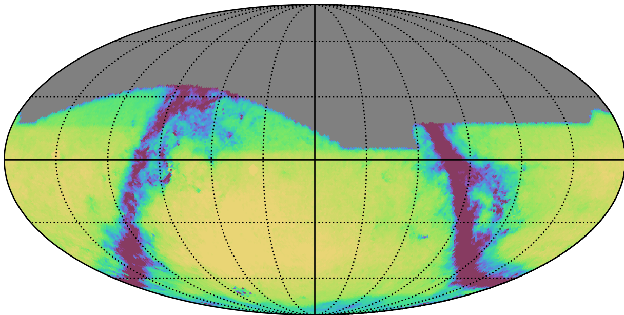
ddf_loaded_fl4_v3.4_10yrs All sky g band: Exgal_CoaddM5
