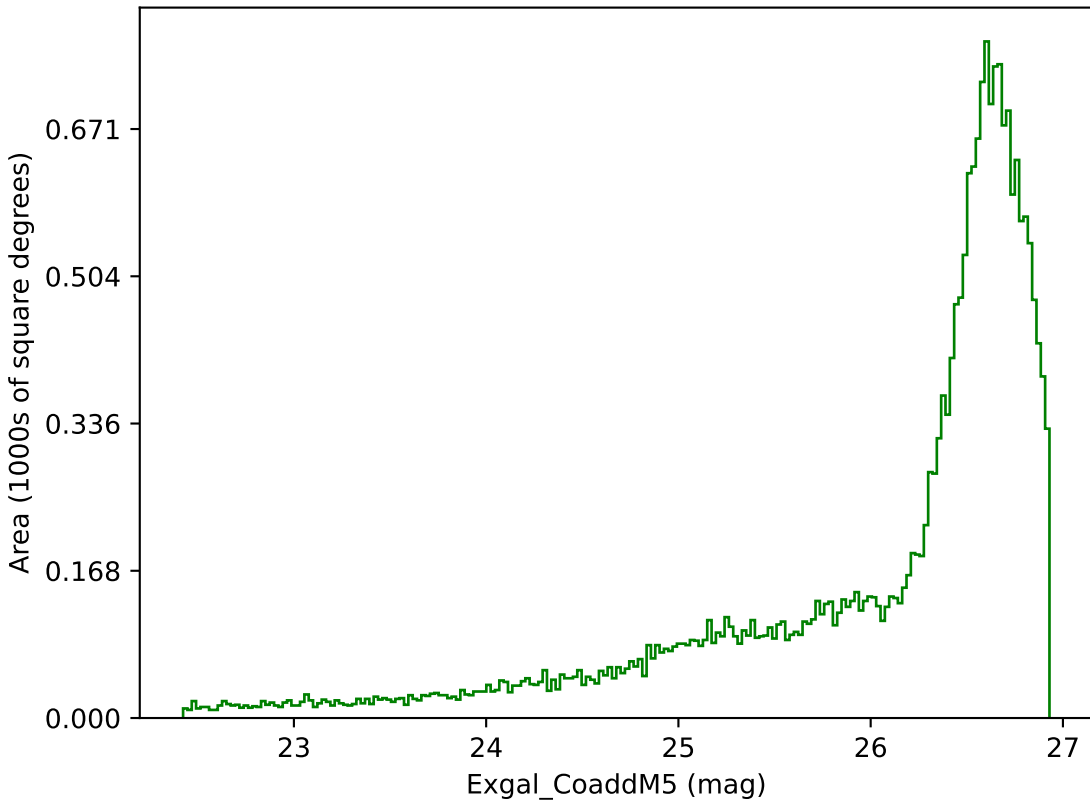
ddf_loaded_fl4_v3.4_10yrs All sky g band: Exgal_CoaddM5
