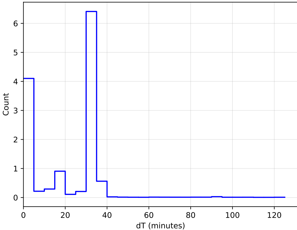
1e6 ddf_loaded_fl4_v3.4_10yrs All sky: DeltaT Histogram
