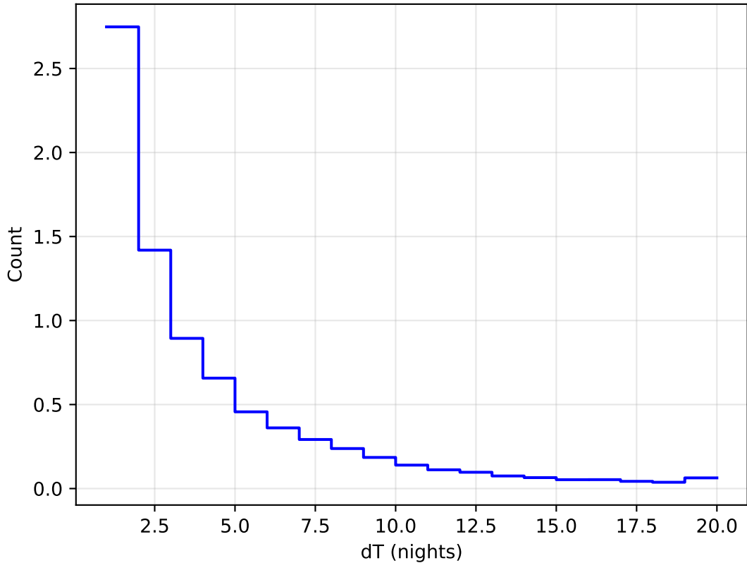
ddf_loaded_fl4_v3.4_10yrs WFD all bands: DeltaNight Histogram 1e6
