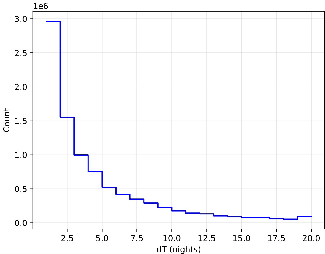
ddf_loaded_fl4_v3.4_10yrs All sky all bands: DeltaNight Histogram
