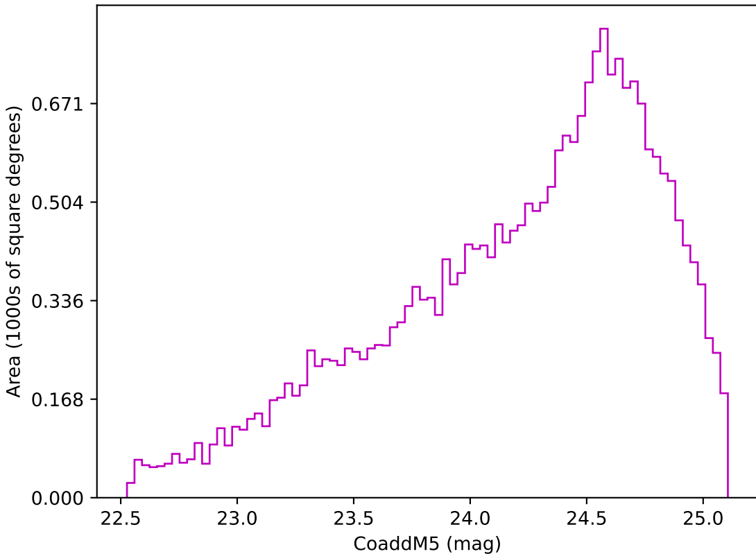
ddf_loaded_fl4_v3.4_10yrs Yr 3-4 z band: CoaddM5
