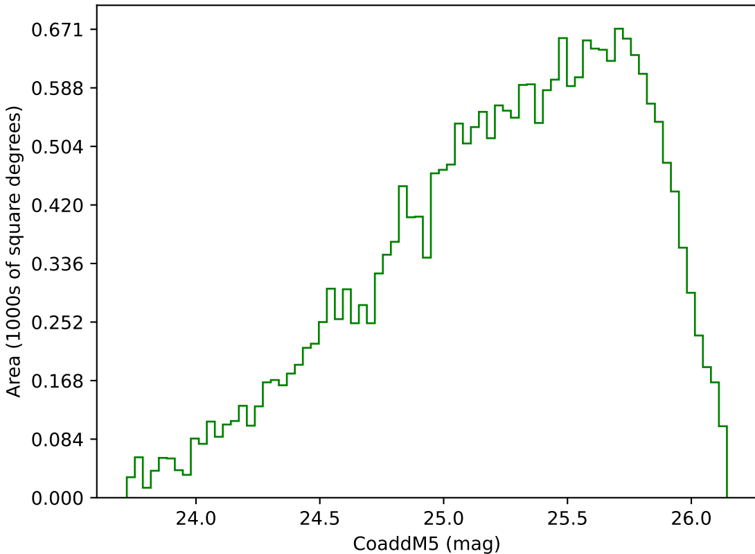
ddf_loaded_fl4_v3.4_10yrs Yr 3-4 g band: CoaddM5
