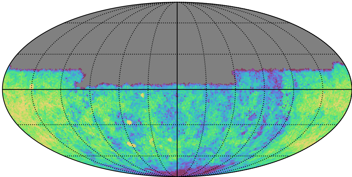
ddf_loaded_fl4_v3.4_10yrs Yr 1 u band: CoaddM5
