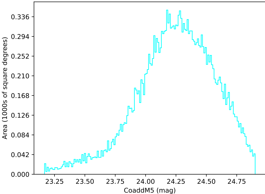
ddf_loaded_fl4_v3.4_10yrs Yr 1 u band: CoaddM5
