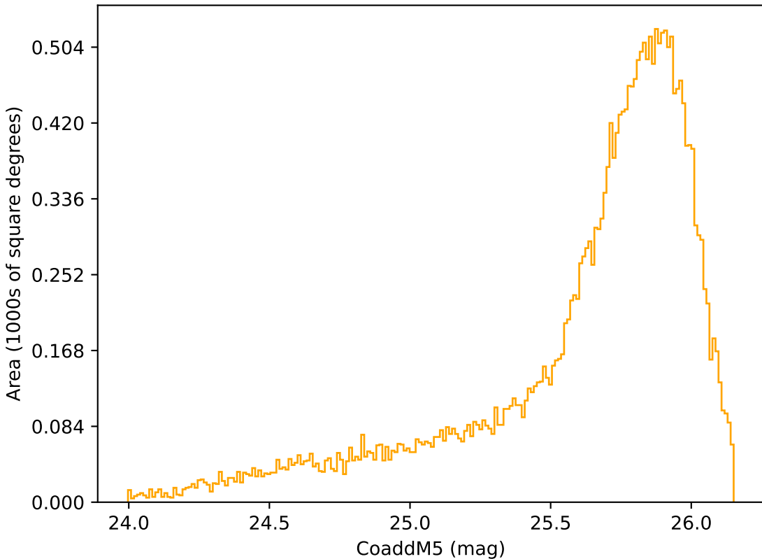
ddf_loaded_fl4_v3.4_10yrs Yr 1 r band: CoaddM5
