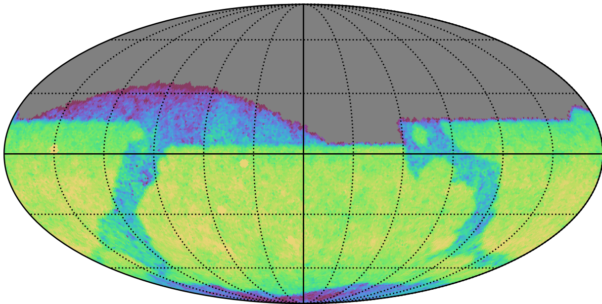
ddf_loaded_fl4_v3.4_10yrs Yr 1 i band: CoaddM5
