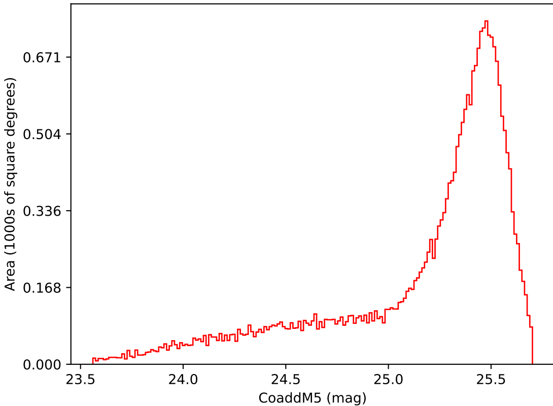
ddf_loaded_fl4_v3.4_10yrs Yr 1 i band: CoaddM5
