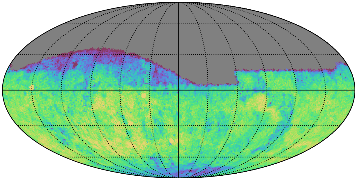
ddf_loaded_fl4_v3.4_10yrs Yr 1 g band: CoaddM5
