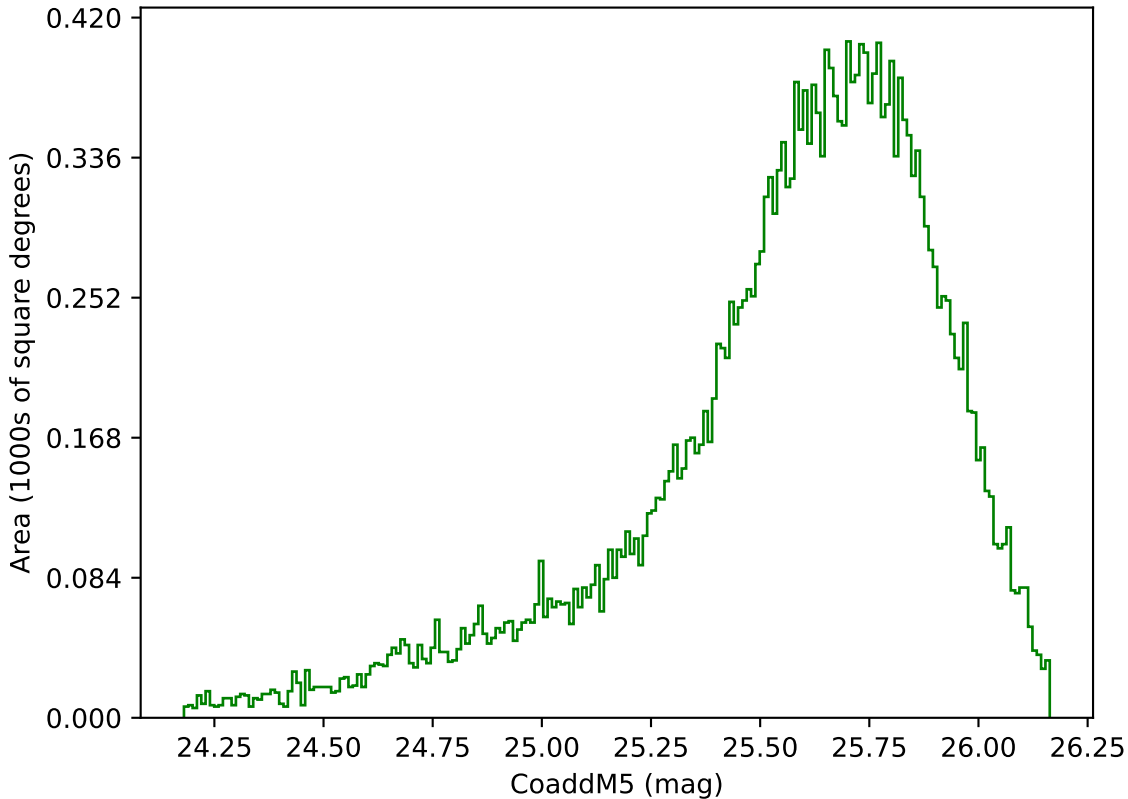
ddf_loaded_fl4_v3.4_10yrs Yr 1 g band: CoaddM5
