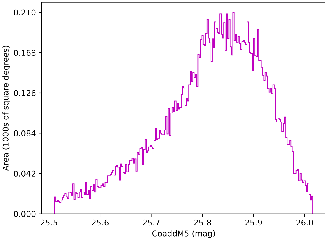
ddf_loaded_fl4_v3.4_10yrs WFD z band: CoaddM5
