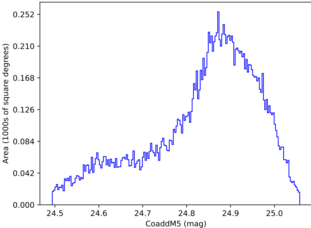
ddf_loaded_fl4_v3.4_10yrs WFD y band: CoaddM5
