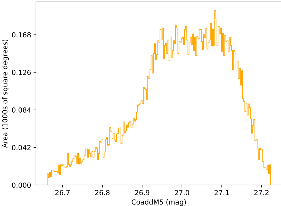
ddf_loaded_fl4_v3.4_10yrs WFD r band: CoaddM5
