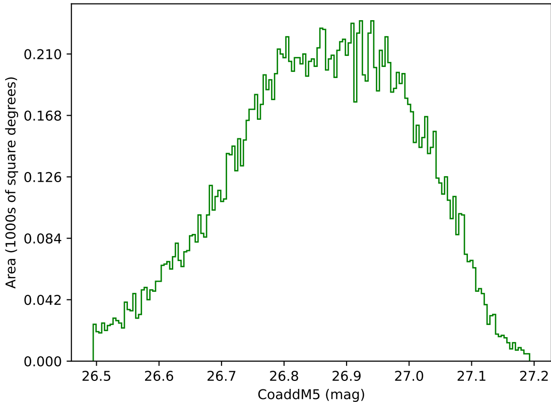
ddf_loaded_fl4_v3.4_10yrs WFD g band: CoaddM5
