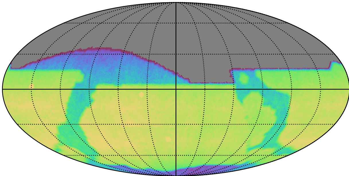
ddf_loaded_fl4_v3.4_10yrs All sky z band: CoaddM5
