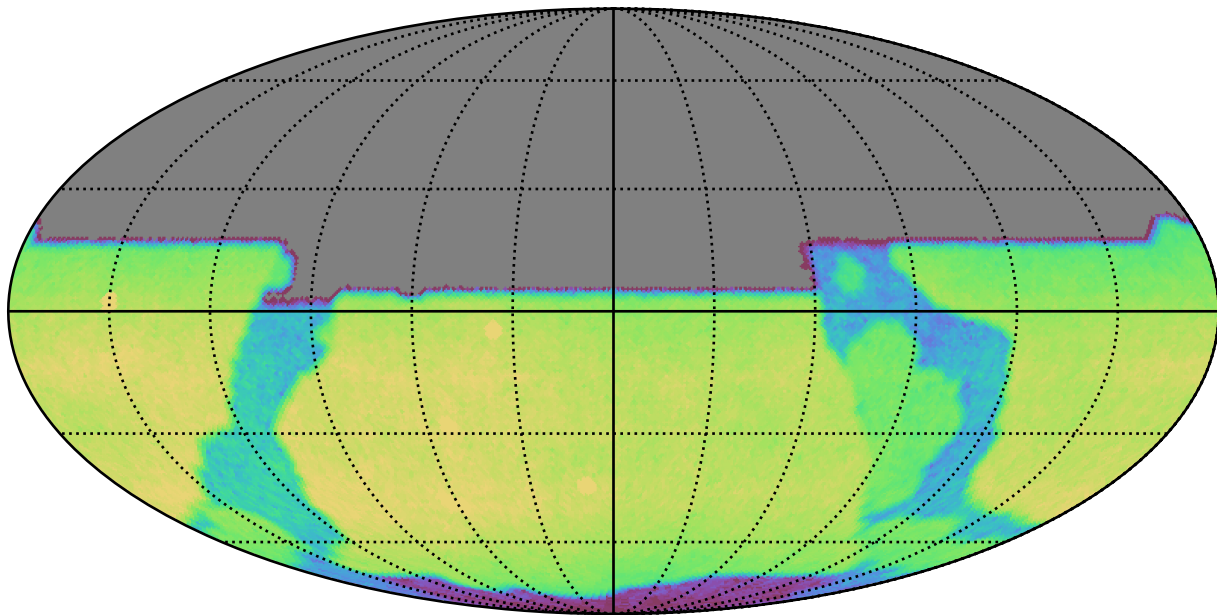
ddf_loaded_fl4_v3.4_10yrs All sky y band: CoaddM5
