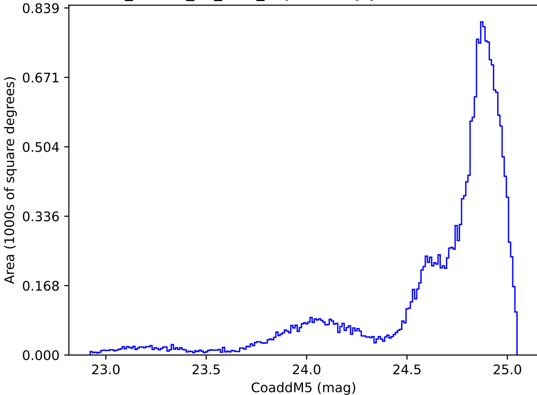
ddf_loaded_fl4_v3.4_10yrs All sky y band: CoaddM5
