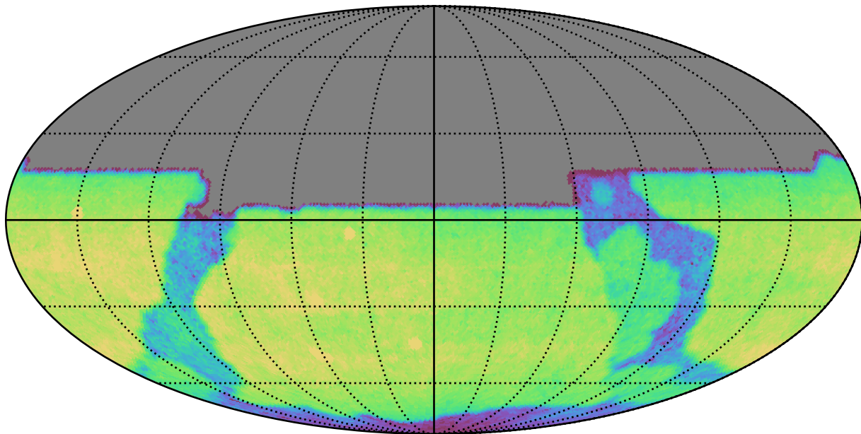
ddf_loaded_fl4_v3.4_10yrs All sky u band: CoaddM5
