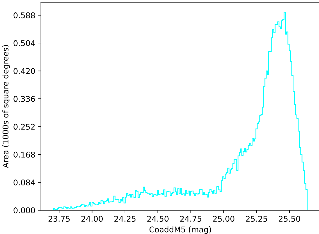
ddf_loaded_fl4_v3.4_10yrs All sky u band: CoaddM5
